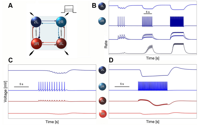
FIG. 6. Validation of slow synaptic dynamics and electrical coupling mechanisms (Fact-check list III). Compare panels C and D with the corresponding neurophysiological recordings presented in Fig. 7 of Ref. 10 . (A–B) Three positive current pulses of progressively increasing amplitude are applied to Si2R to calibrate the \alpha -synapse and logistic synapse models (bottom trace) and to reproduce the inhibitory postsynaptic potential (IPSP) responses observed in the contralateral Si2L (top trace in panel B). (C–D) Two positive current pulses injected into Si2R evoke accumulating IPSP responses in Si2L (top trace) and elicit both fast and slow echo responses in Si3L. These echoes arise from distinct mechanisms: a fast component mediated by the electrical coupling and a slower, delayed inhibitory response mediated by the logistic synapse between Si2R and Si3L. Together, these features reproduce the experimentally observed dynamics and confirm the functional roles of electrical and chemical inhibition within the swim CPG circuitry (see Fig. 2A).
